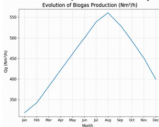
Figure 3. Evolution of biogas production as a function of time
