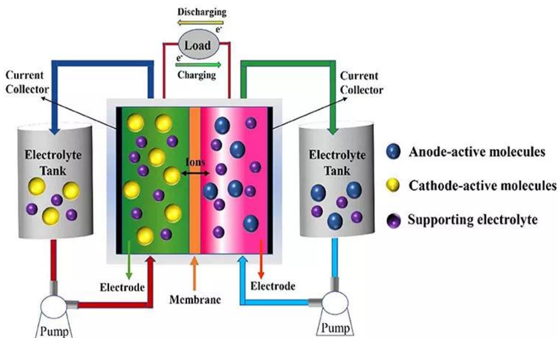
Fig. 2. Flow type or flux type battery
