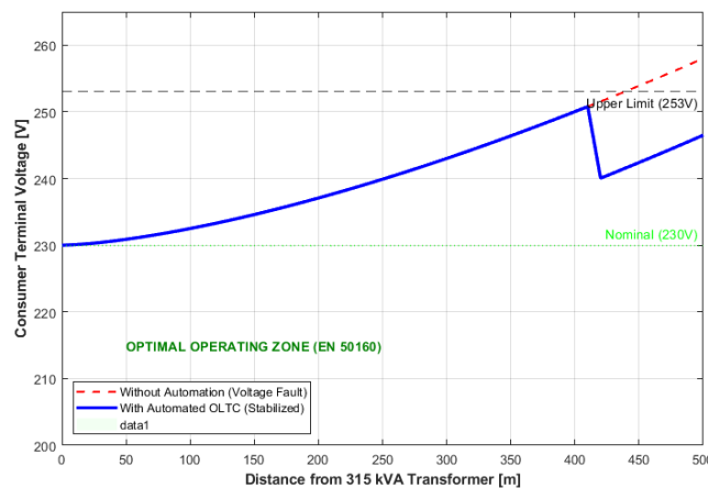
Figure 3. Comparative analysis of voltage stabilization performance through the automated OLTC system
